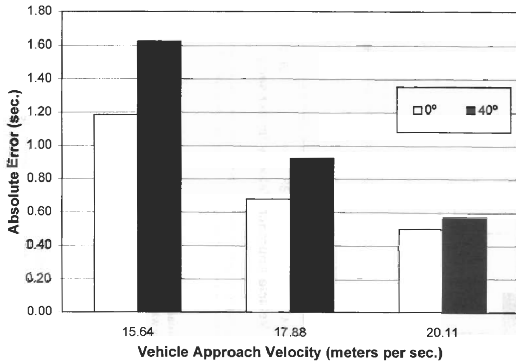
FIGURE 7 Interaction between vehicle approach trajectory and vehicle approach velocity for absolute error. Note that when the vehicle approach velocity is increased for both approach trajectories, there is also an increase in estimates of T_e .
